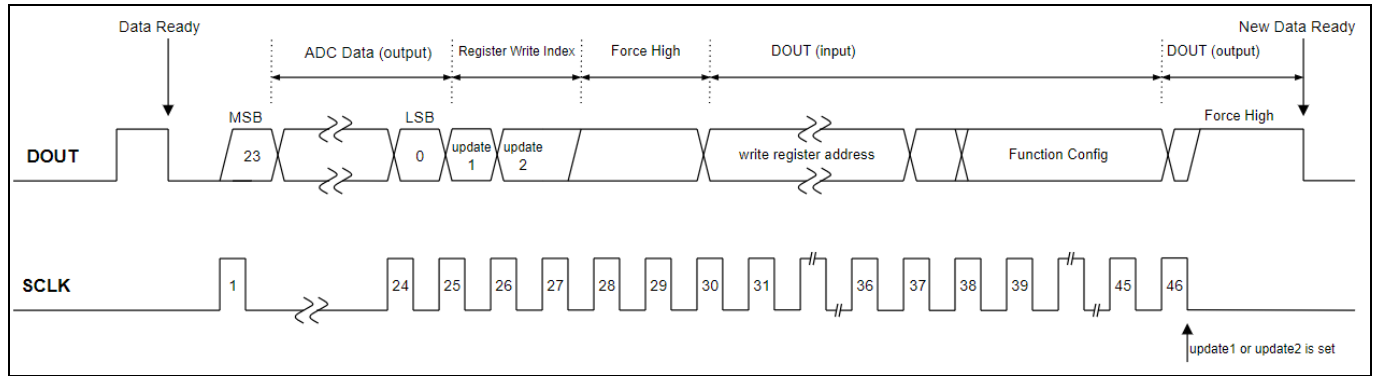
Figure 10: Timing diagram of PMD040B configuration (write procedure).
