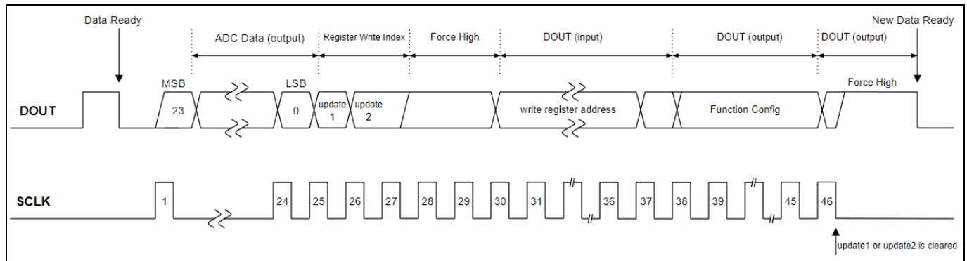
Figure 11: Timing diagram of PMD040B configuration (read procedure).
